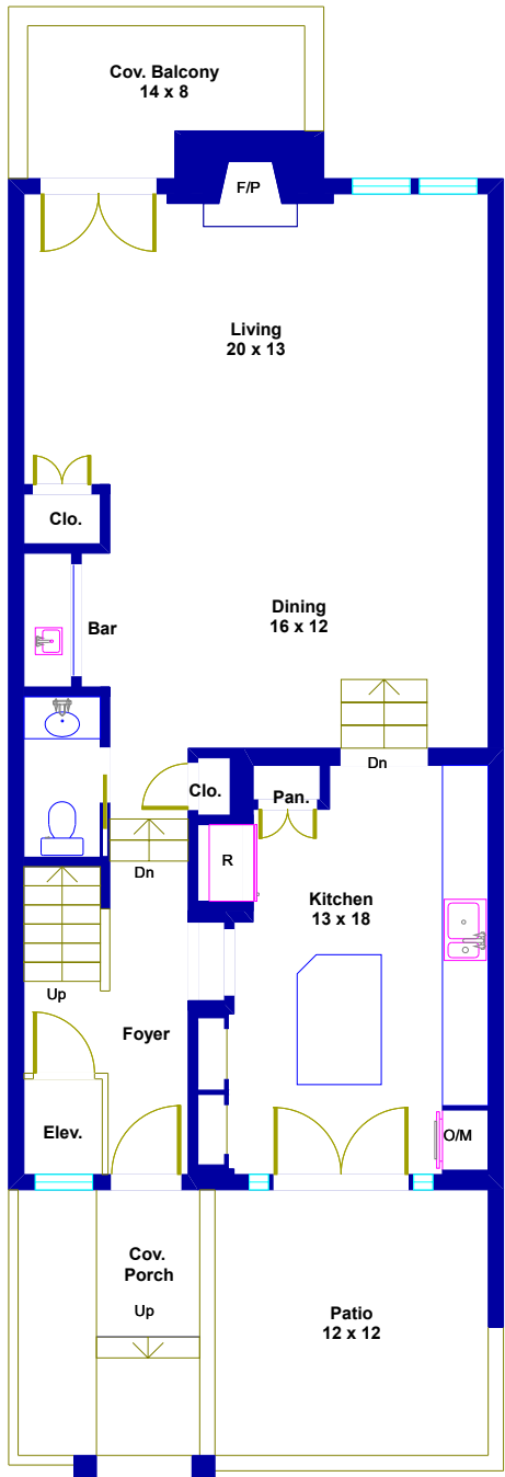
Condominium First Floor
